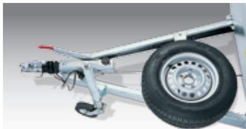
Spare wheel holder mounted on drawbar (only for longer drawbars)
